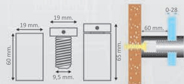
ALU MAGNUM 1960 cod. 100420
