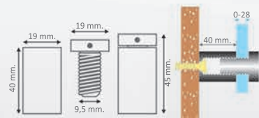
ALU MAGNUM 1940 cod. 100418
